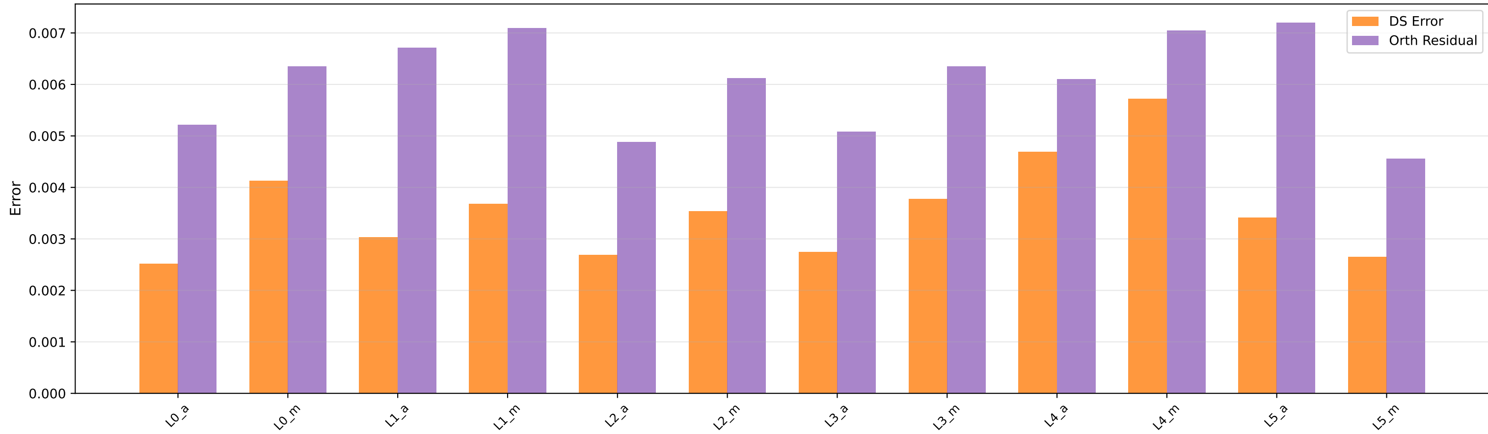
Setting B - Per-Layer Diagnostics at iter 5000 (setting_b_orthostochastic_optimized_seed1)
