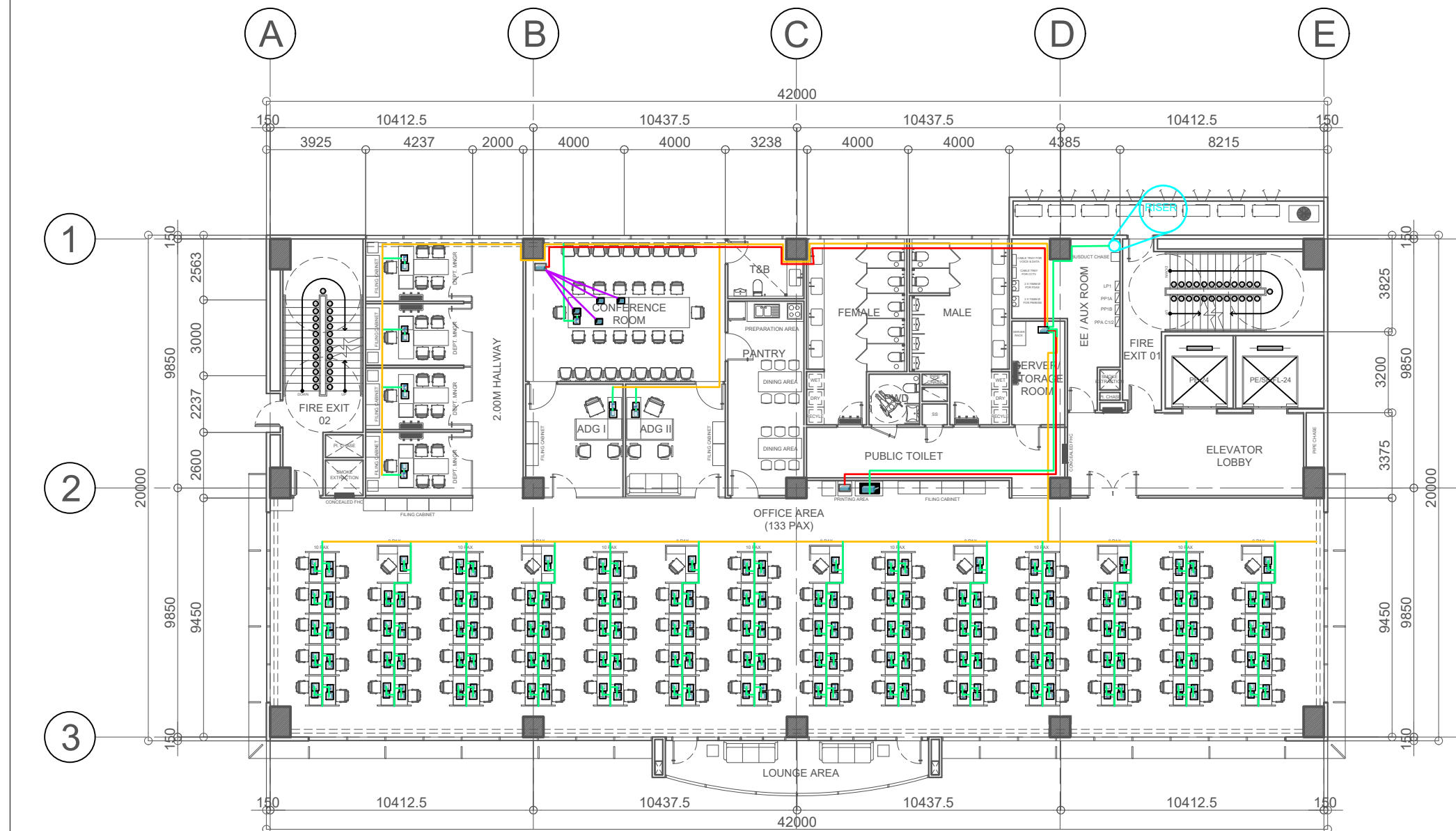
THIRD FLOOR PLAN SCALE: 1:100 MTS
