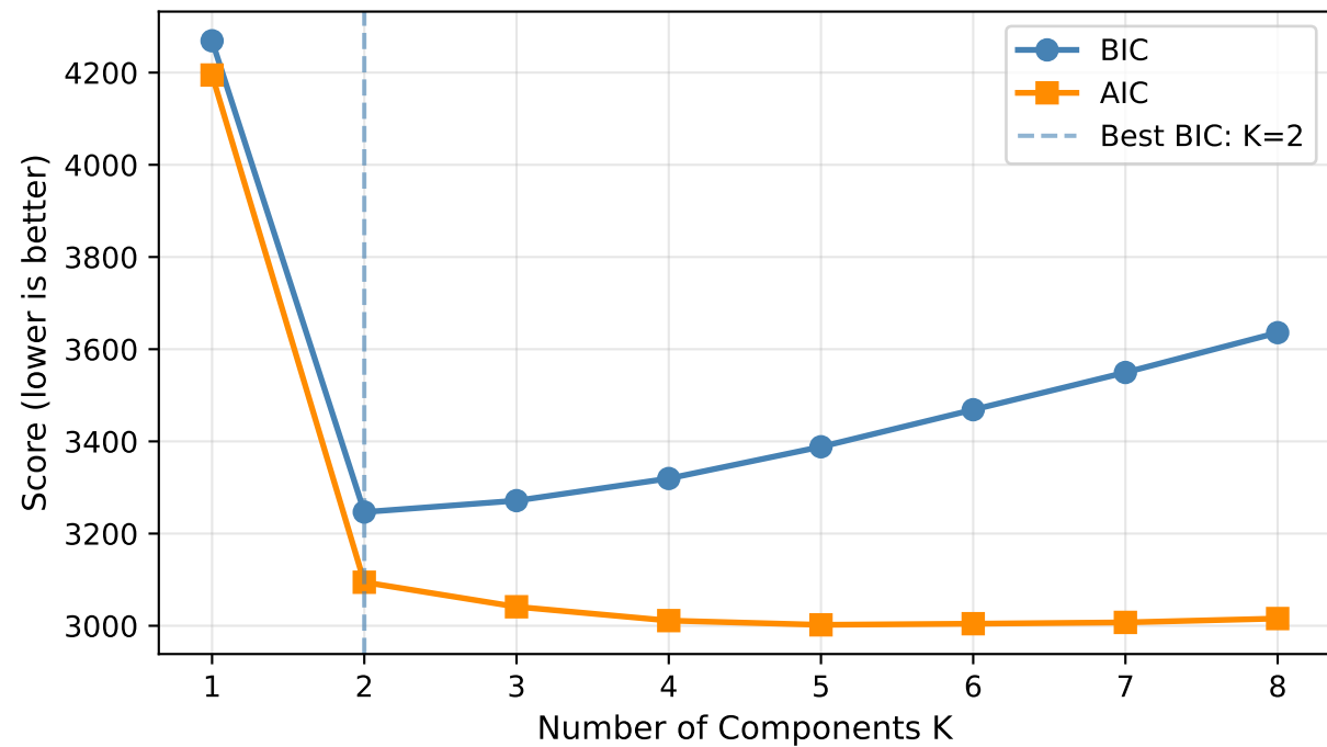
(a) BIC & AIC vs K
