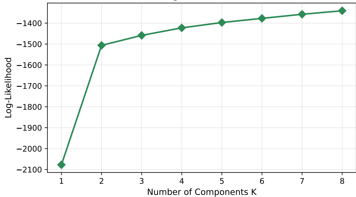
(b) Log-Likelihood vs K
