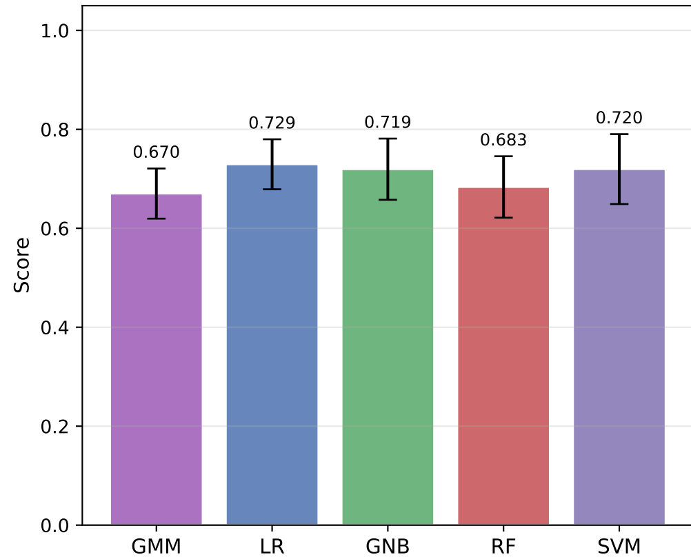
Accuracy
