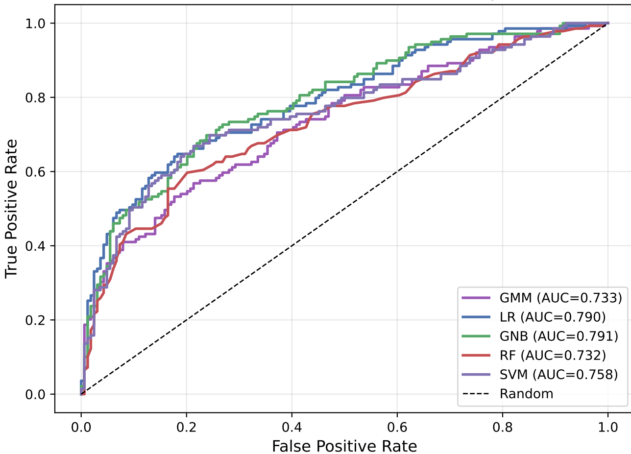
ROC Curves — GMM Classifier vs Baselines (5-fold CV, continuous features only)
