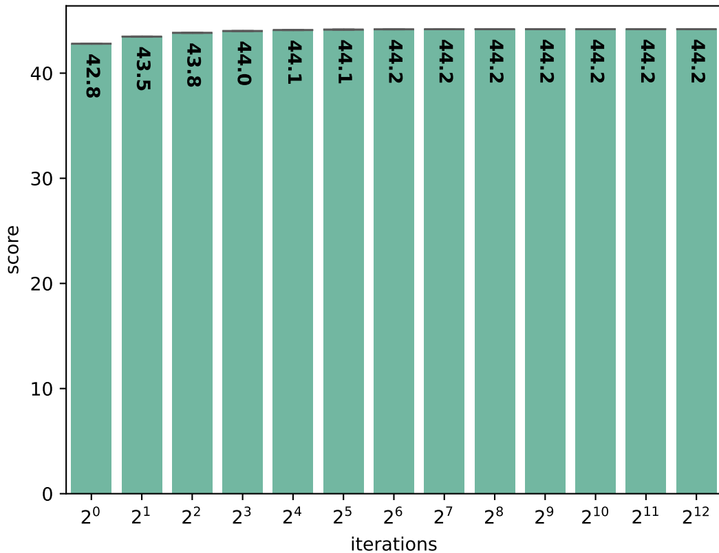
ACAE: Dhrystone score (in DMIPS)
