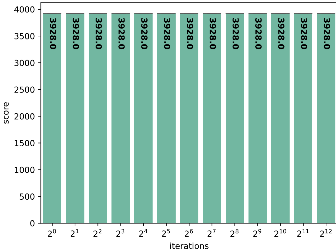
ACAE: Embench-cubic score (in \mu\text{s}/\text{iteration} )
