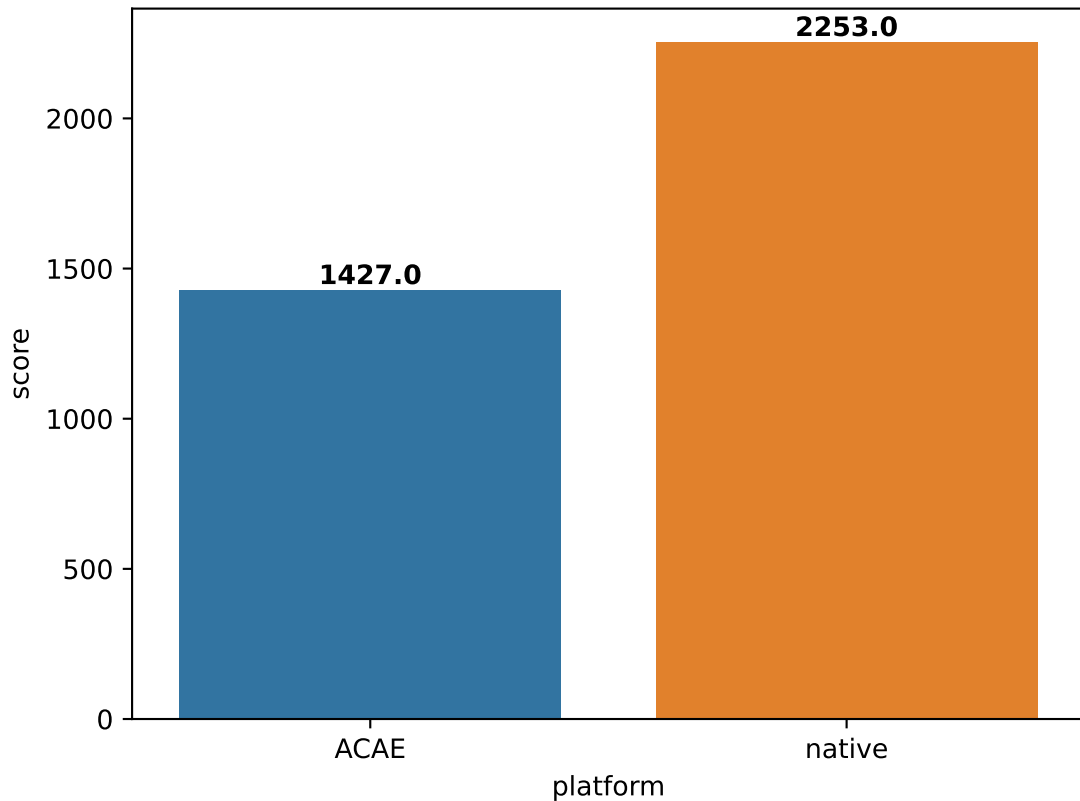
Embench-edn score (in \mu\text{s}/\text{iteration} )
