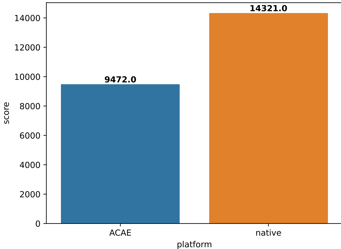
Embench-huffbench score (in \mu\text{s}/\text{iteration} )
