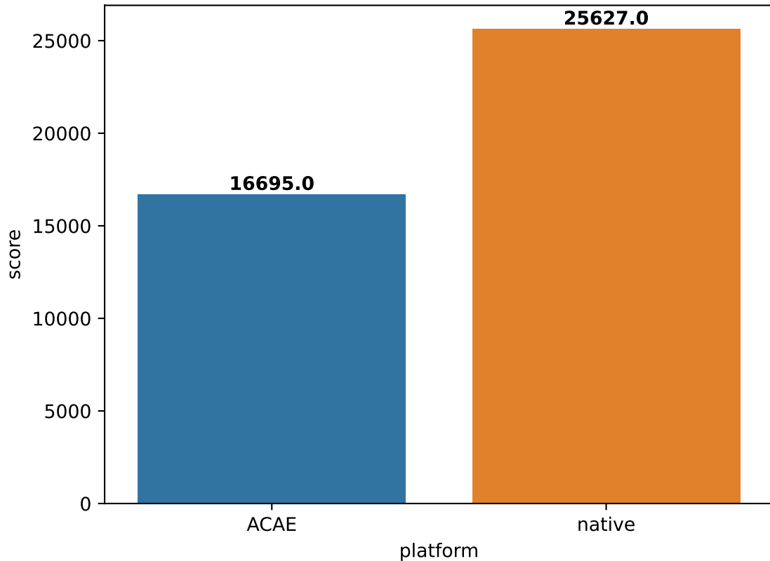
Embench-picojpeg score (in \mu\text{s}/\text{iteration} )
