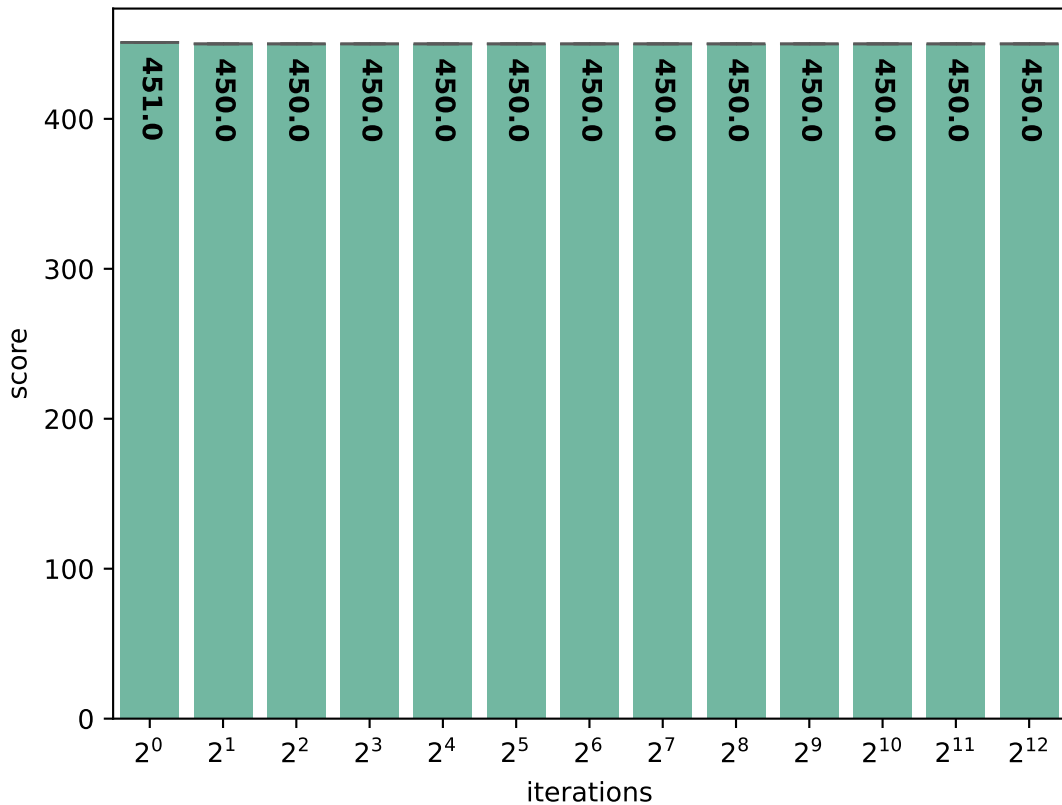
native: Embench-aha-mont64 score (in \mu\text{s}/\text{iteration} )
