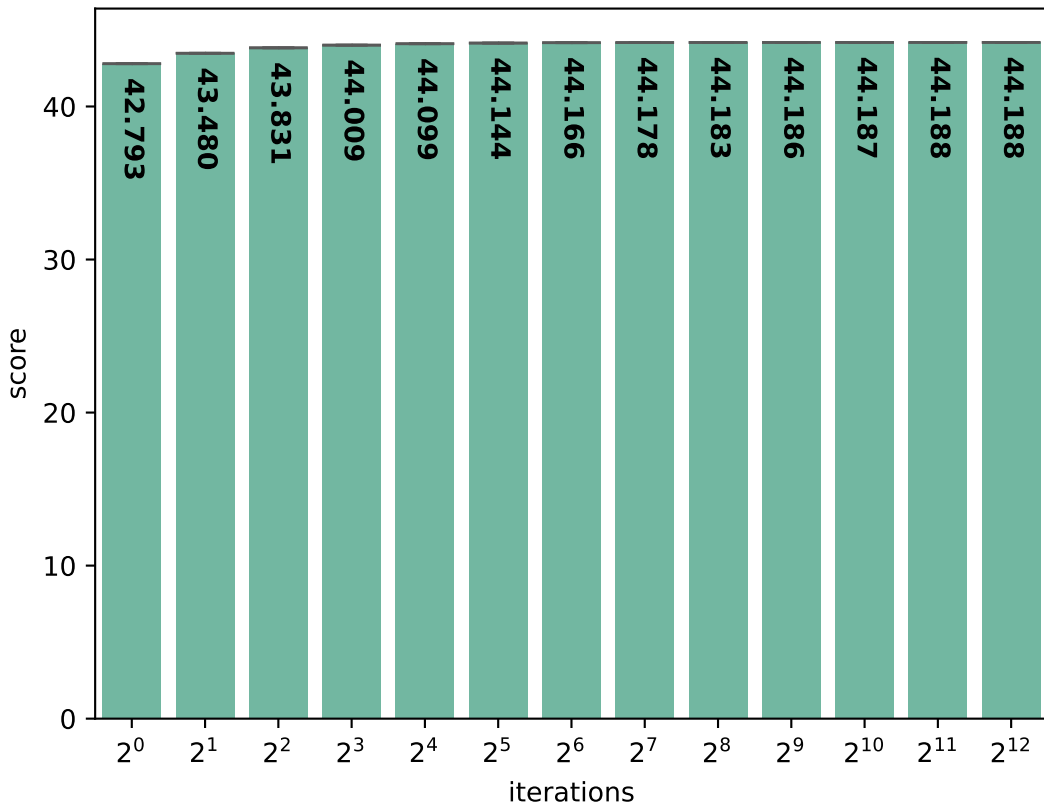
ACAE: Dhrystone score (in DMIPS)
