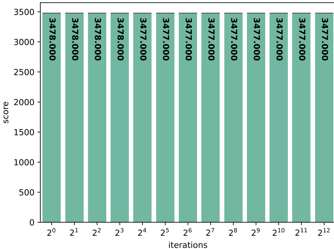
ACAE: Embench-matmult-int score (in \mu\text{s}/\text{iteration} )
