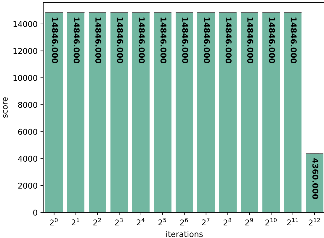
ACAE: Embench-qduino score (in \mu\text{s}/\text{iteration} )
