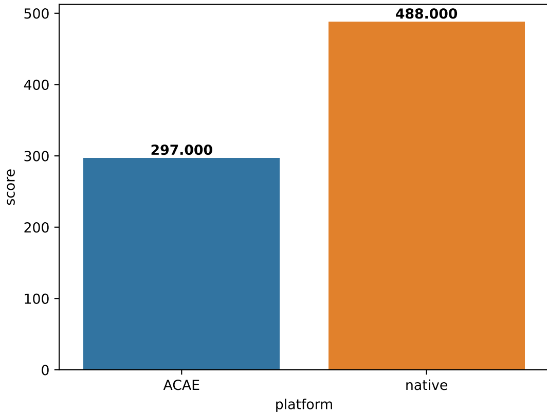
Embench-crc32 score (in \mu\text{s}/\text{iteration} )
