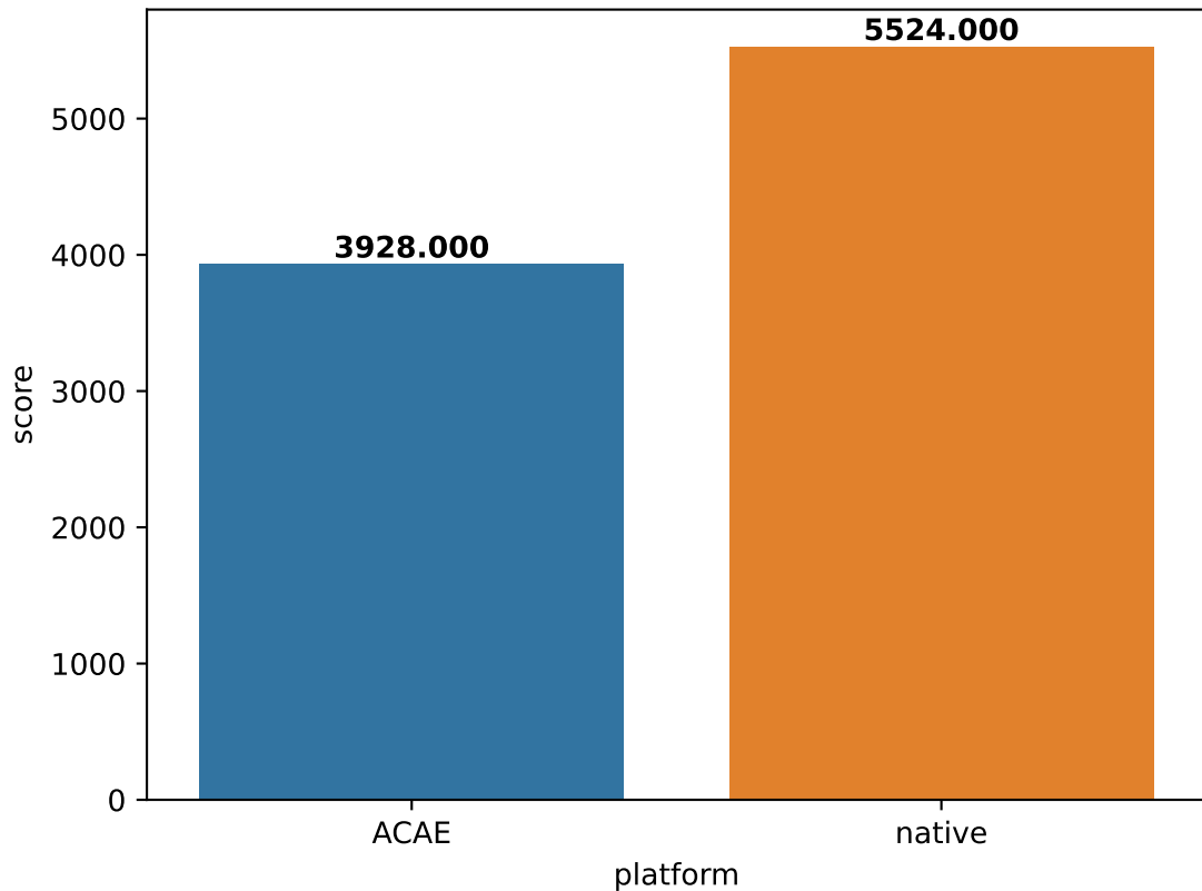
Embench-cubic score (in \mu\text{s}/\text{iteration} )
