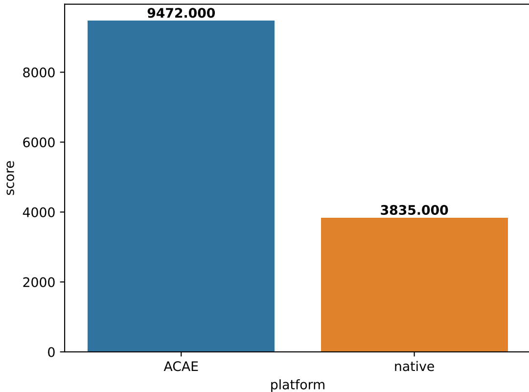
Embench-huffbench score (in \mu\text{s}/\text{iteration} )
