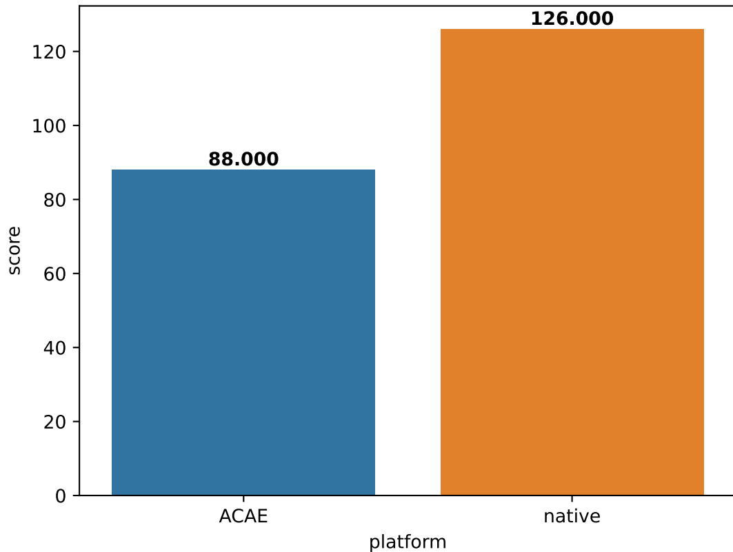
Embench-minver score (in \mu\text{s}/\text{iteration} )
