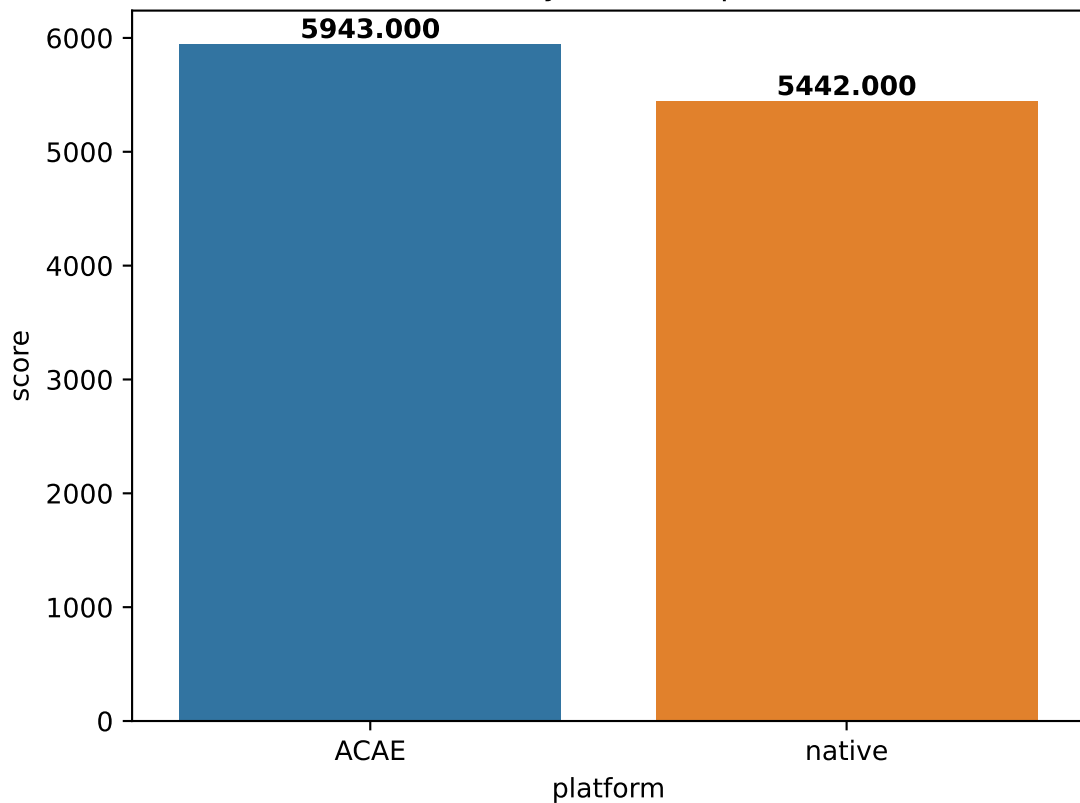
Embench-nbody score (in \mu\text{s}/\text{iteration} )
