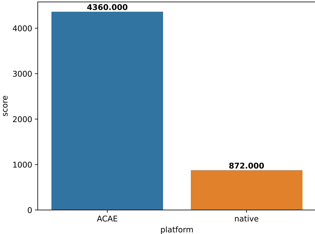
Embench-qduino score (in \mu\text{s}/\text{iteration} )
