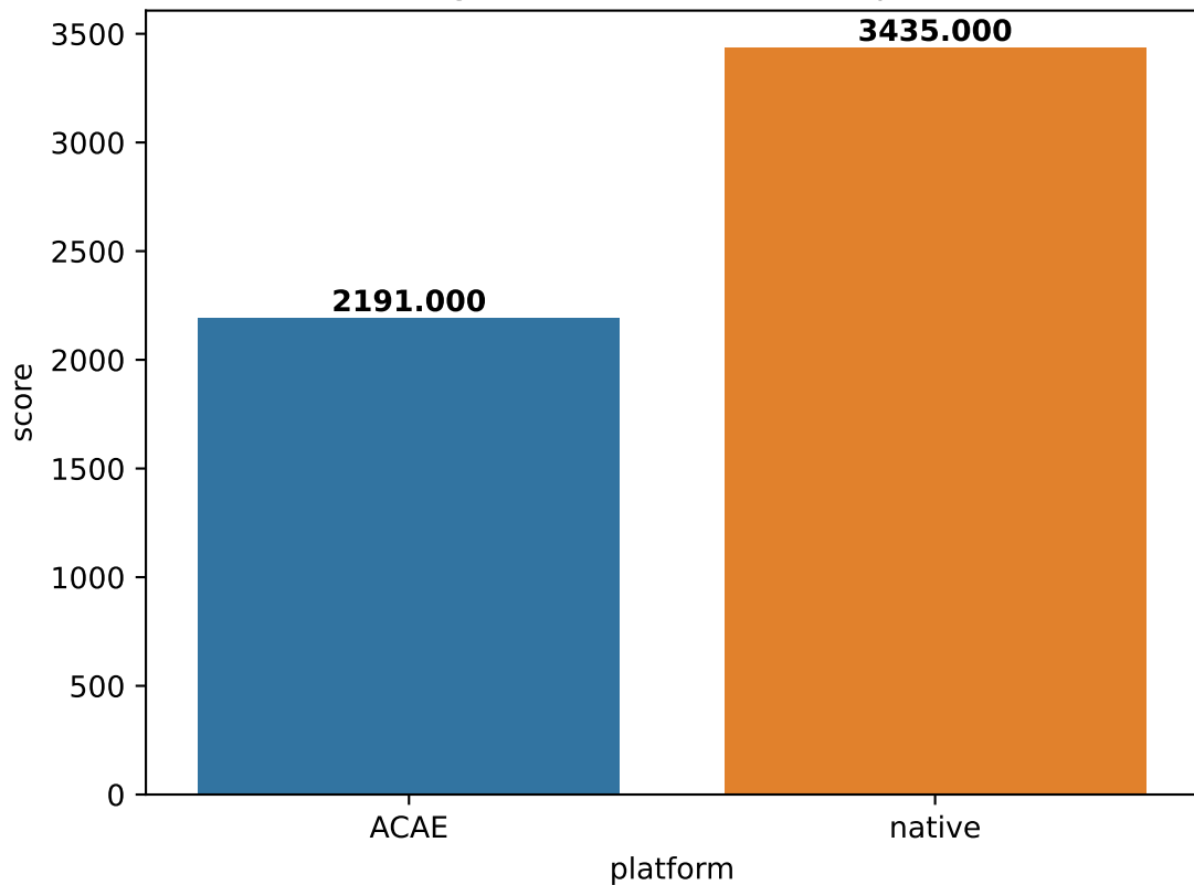
Embench-sglib-combined score (in \mu\text{s}/\text{iteration} )
