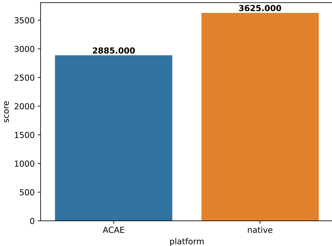
Embench-st score (in \mu\text{s}/\text{iteration} )
