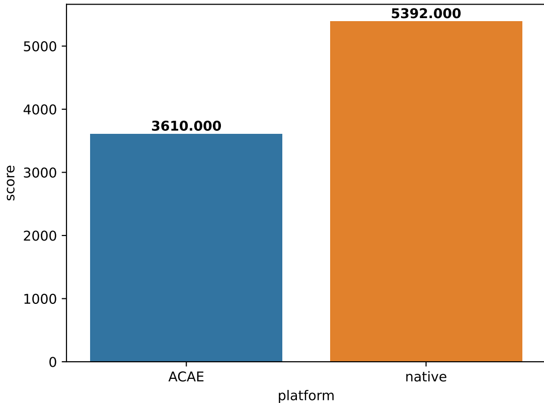
Embench-wikisort score (in \mu\text{s}/\text{iteration} )
