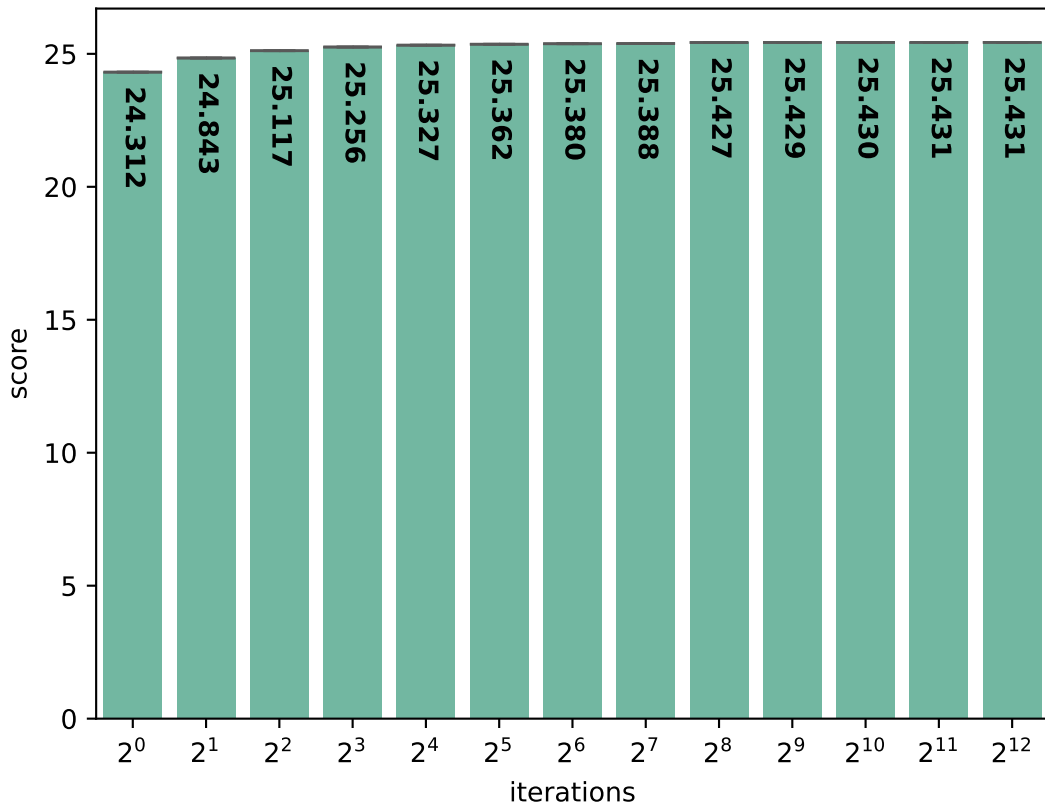
native: Dhrystone score (in DMIPS)
