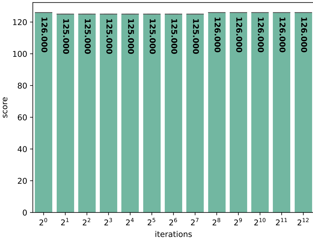
native: Embench-minver score (in \mu\text{s}/\text{iteration} )
