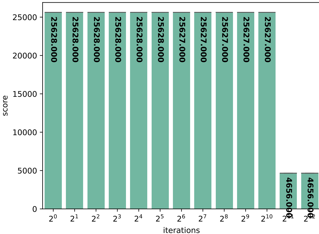
native: Embench-picojpeg score (in \mu\text{s}/\text{iteration} )
