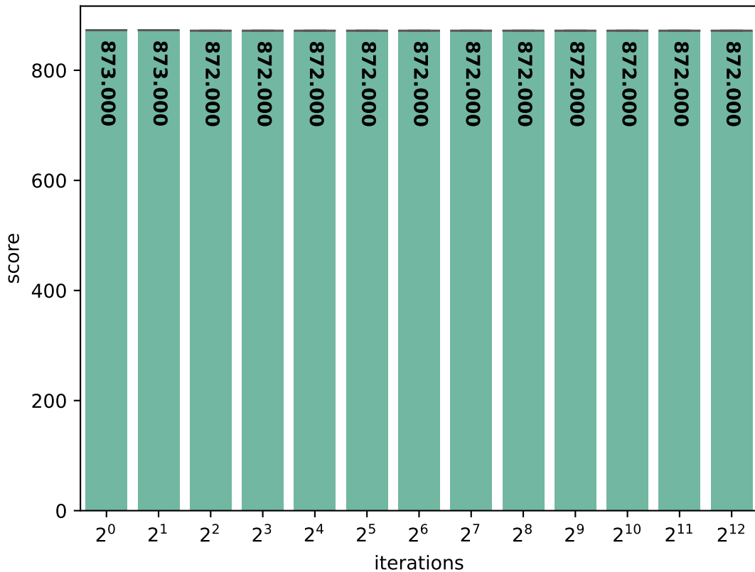
native: Embench-slre score (in \mu\text{s}/\text{iteration} )
