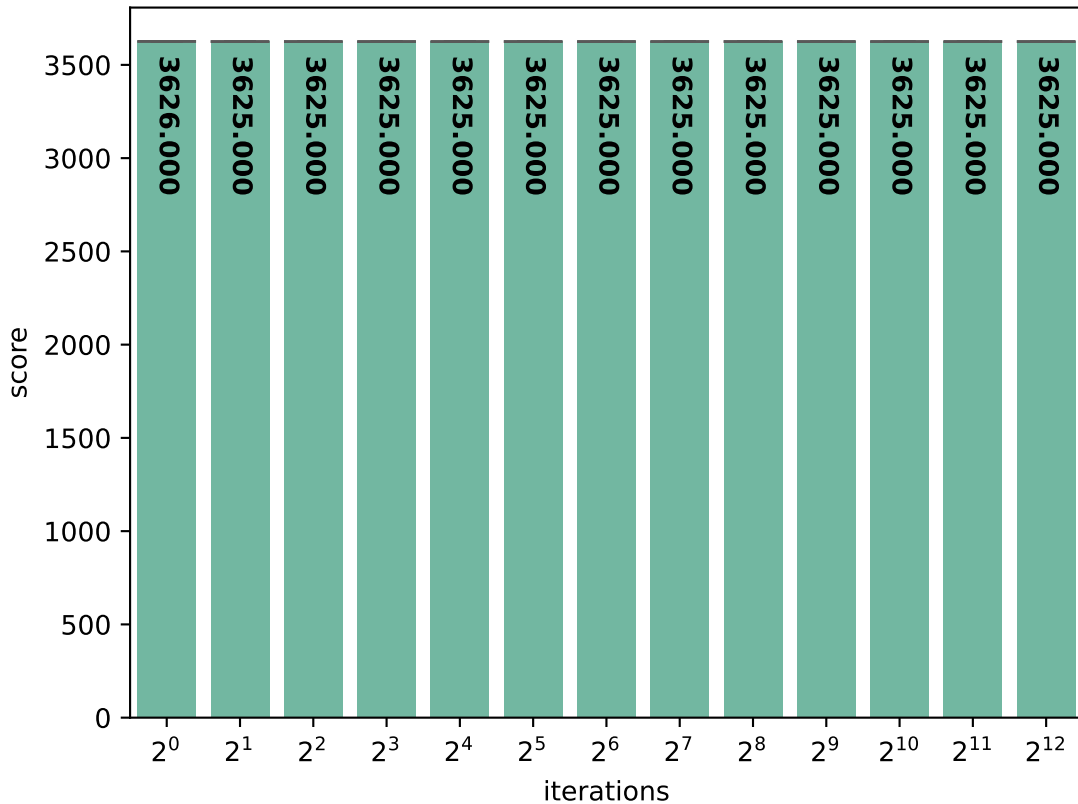
native: Embench-st score (in \mu\text{s}/\text{iteration} )
