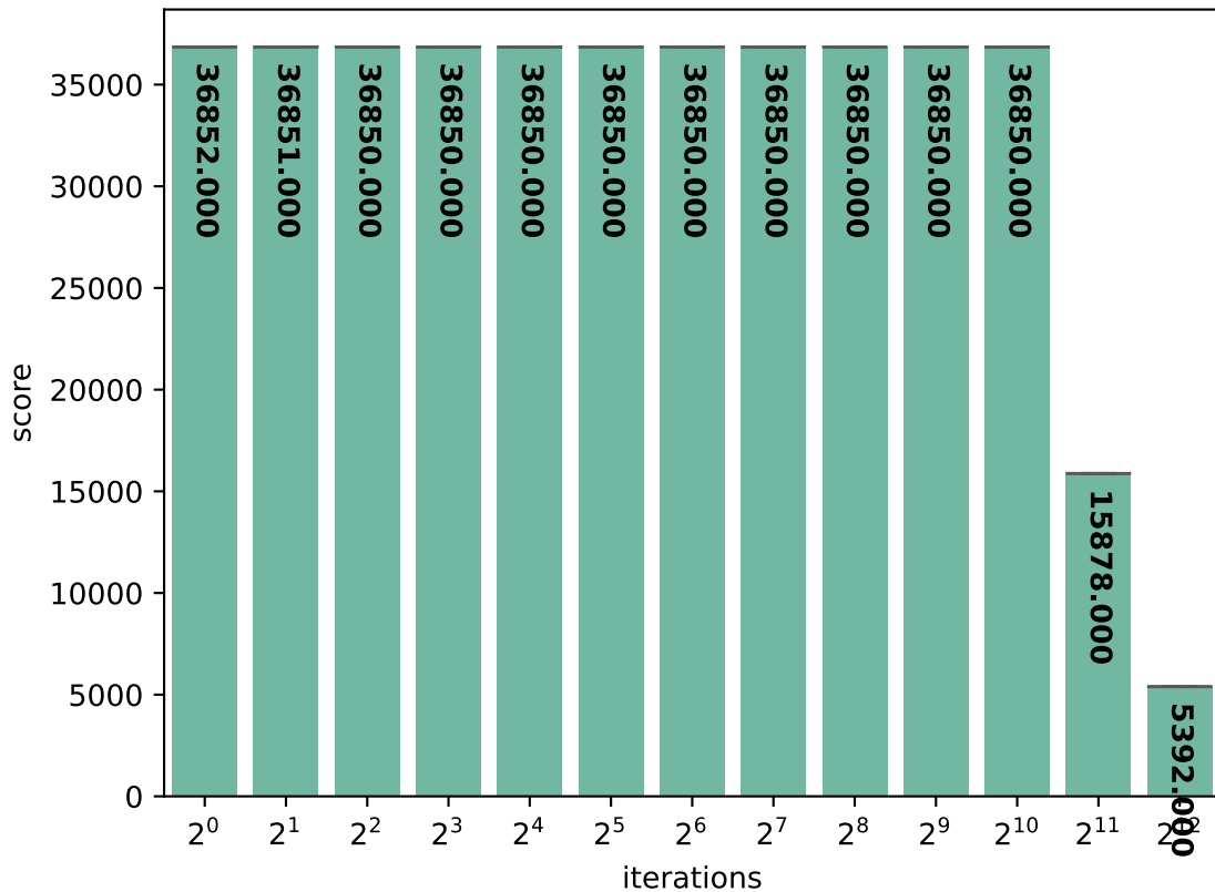
native: Embench-wikisort score (in \mu\text{s}/\text{iteration} )
