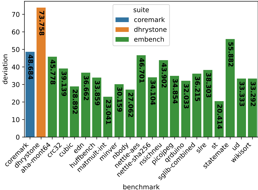
Deviation of ACAE relative to native (in %)
