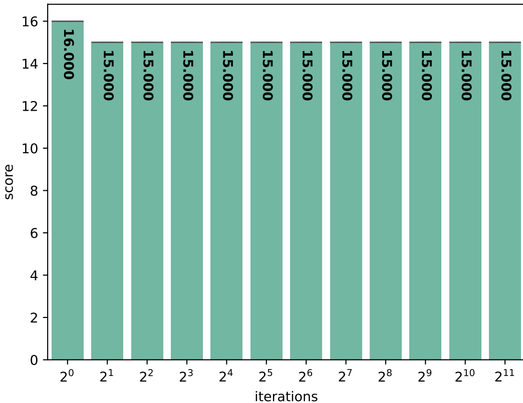
ACAE: Embench-statestate score (in \mu\text{s}/\text{iteration} )
