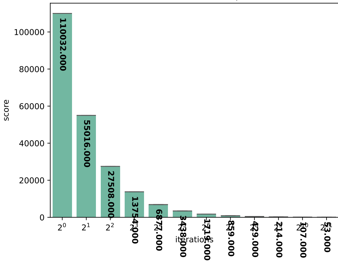
ACAE: Embench-ud score (in \mu\text{s}/\text{iteration} )
