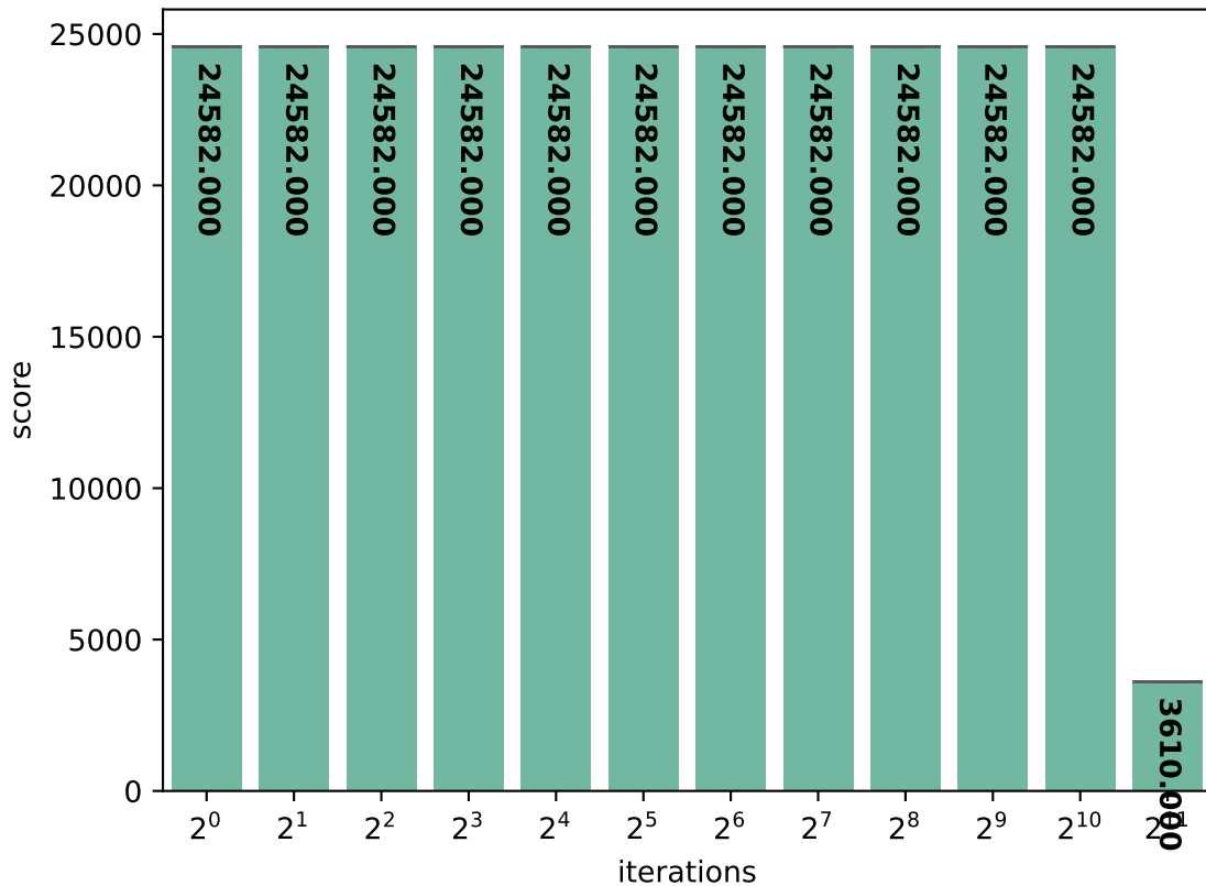
ACAE: Embench-wikisort score (in \mu\text{s}/\text{iteration} )
