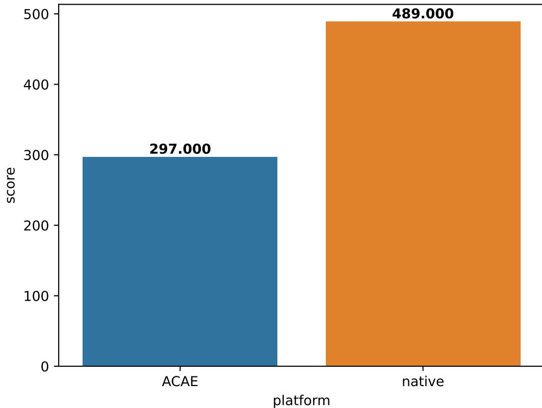
Embench-crc32 score (in \mu s/iteration)
