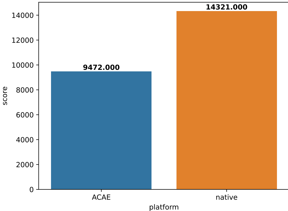
Embench-huffbench score (in \mu\text{s}/\text{iteration} )
