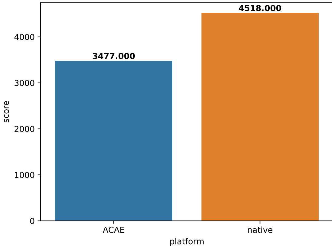
Embench-matmult-int score (in \mu\text{s}/\text{iteration} )
