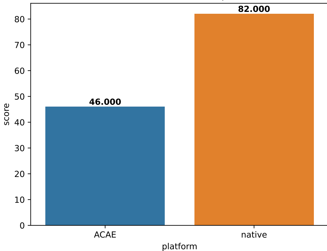
Embench-nsichneu score (in \mu\text{s}/\text{iteration} )
