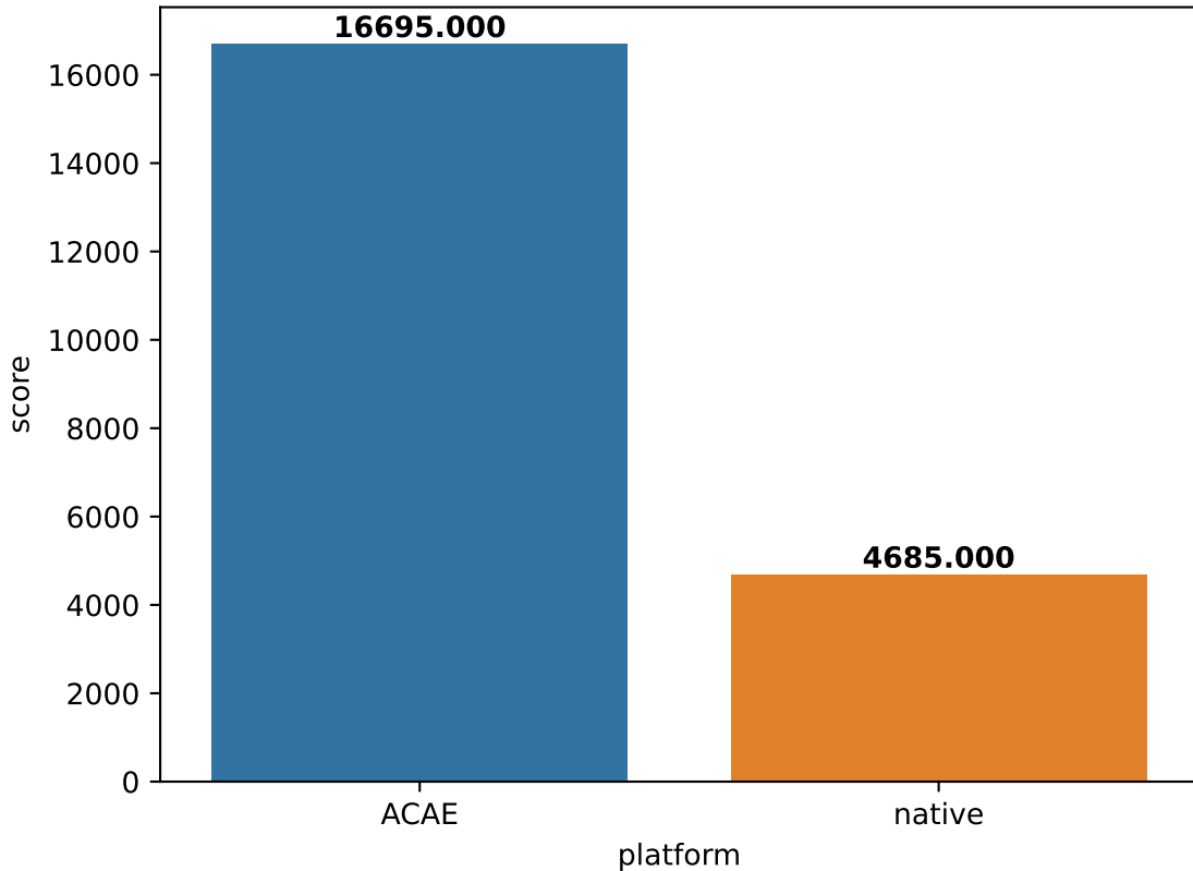
Embench-picojpeg score (in \mu\text{s}/\text{iteration} )
