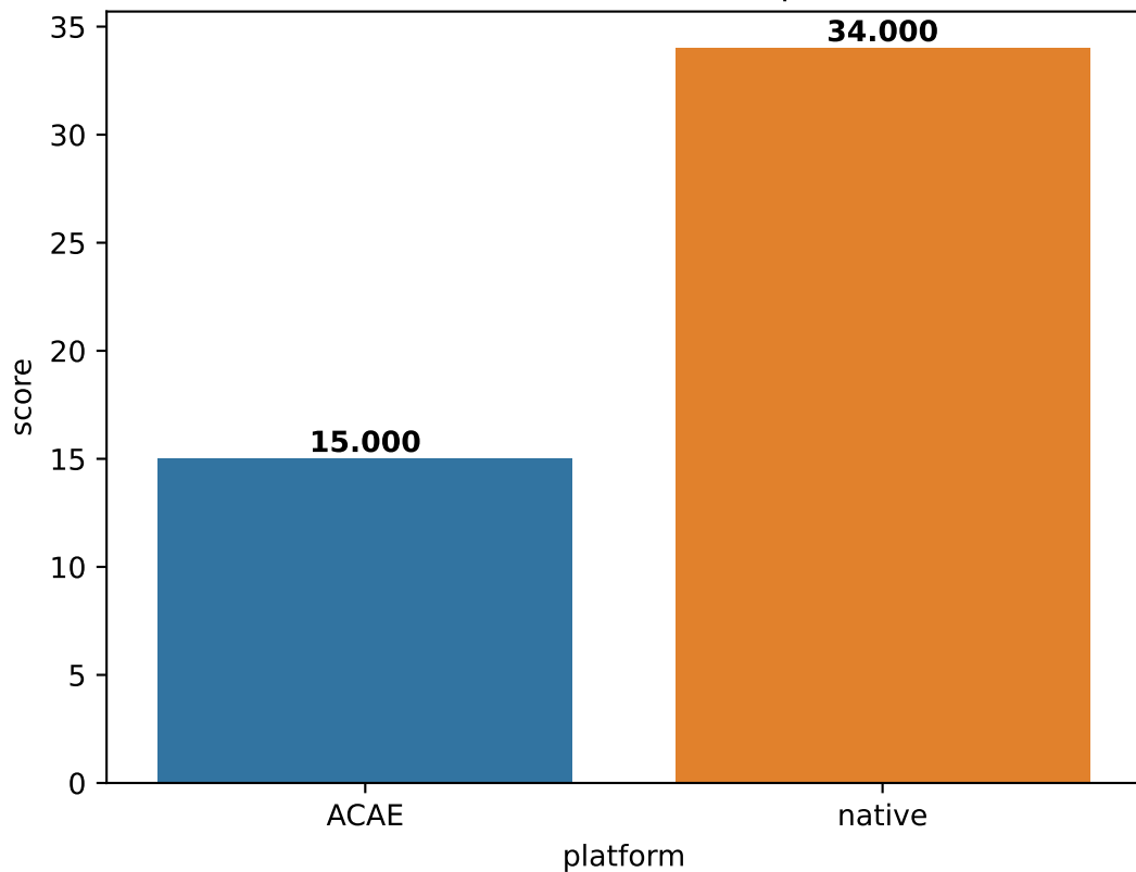
Embench-statestate score (in \mu\text{s}/\text{iteration} )
