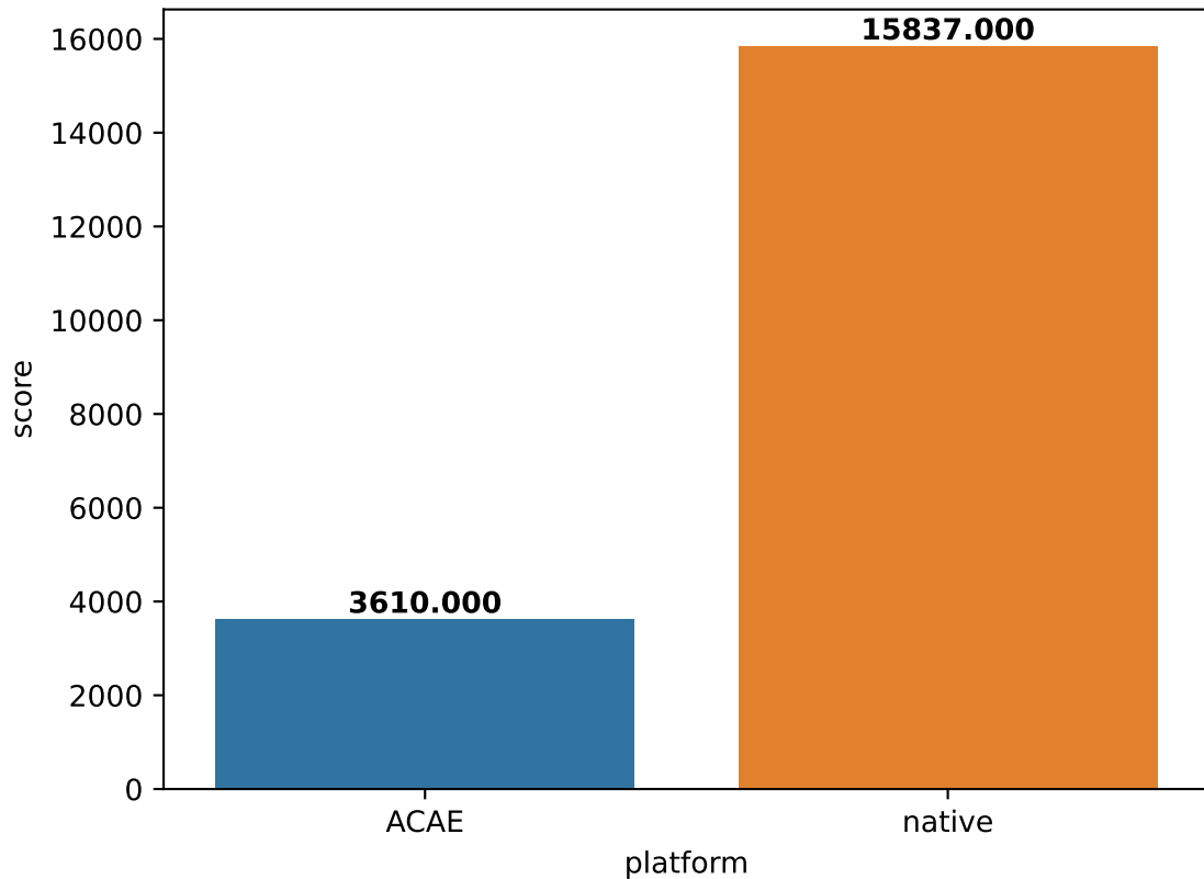
Embench-wikisort score (in \mu\text{s}/\text{iteration} )
