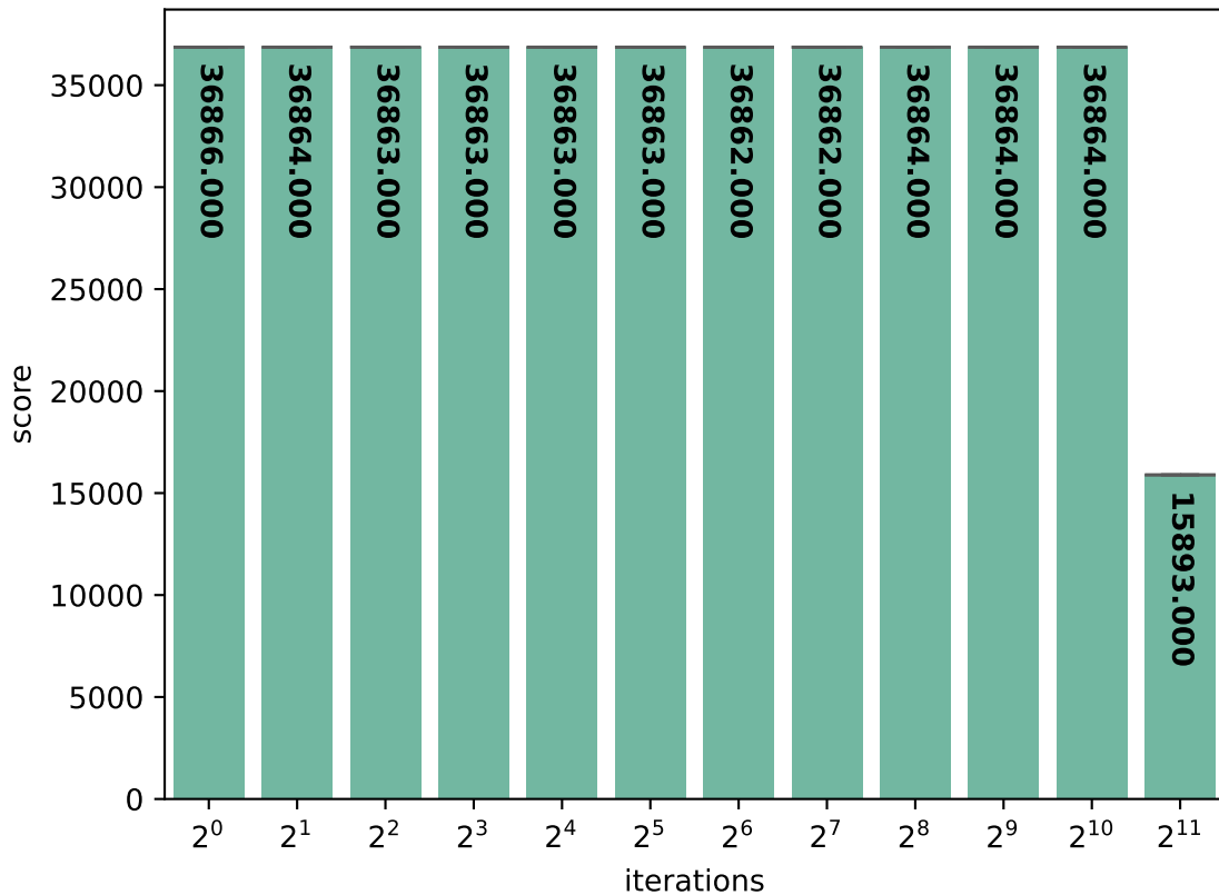
native: Embench-nbody score (in \mu\text{s}/\text{iteration} )
