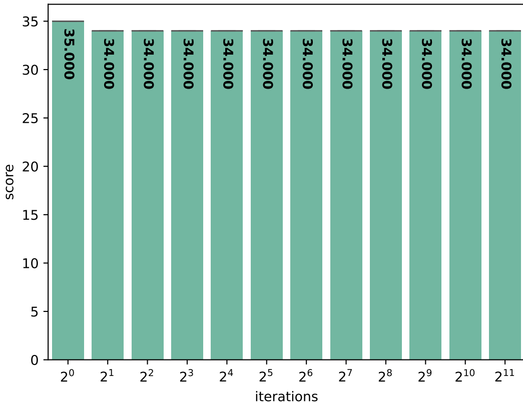
native: Embench-statestate score (in \mu\text{s}/\text{iteration} )
