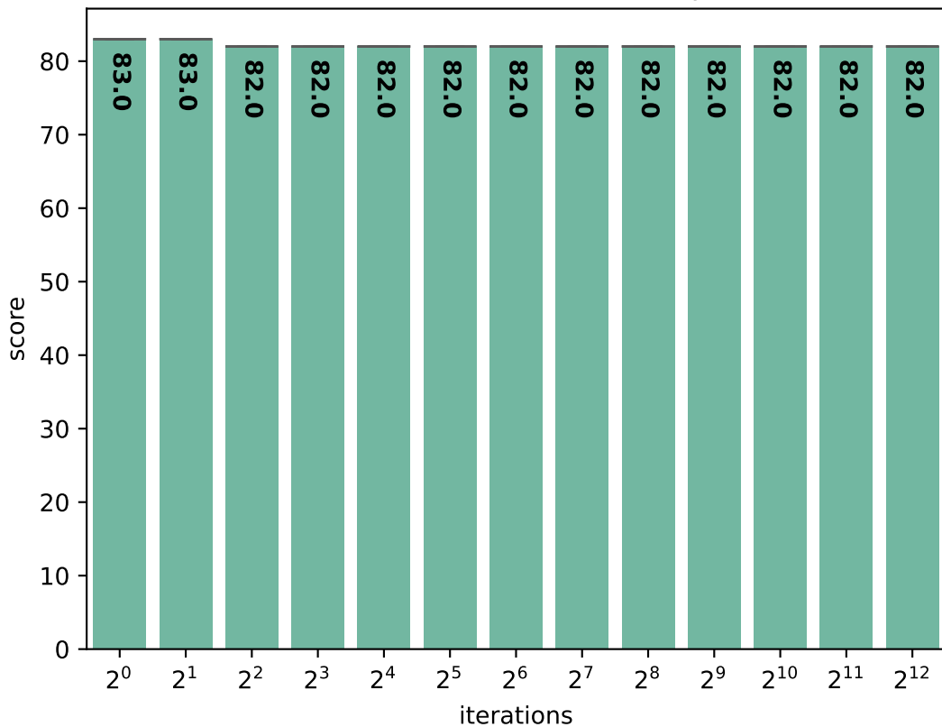
native: Embench-nsichneu score (in \mu\text{s}/\text{iteration} )
