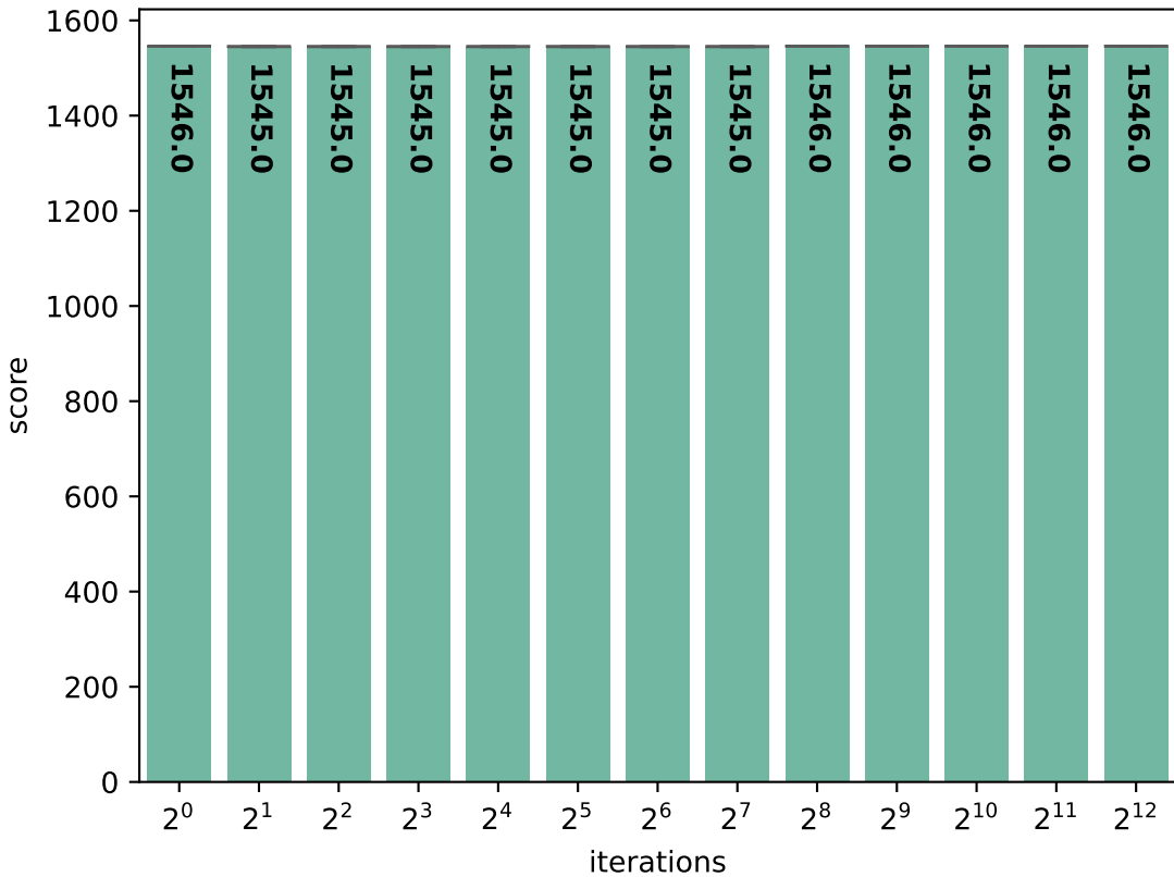
native: Embench-nettle-aes score (in \mu\text{s}/\text{iteration} )
