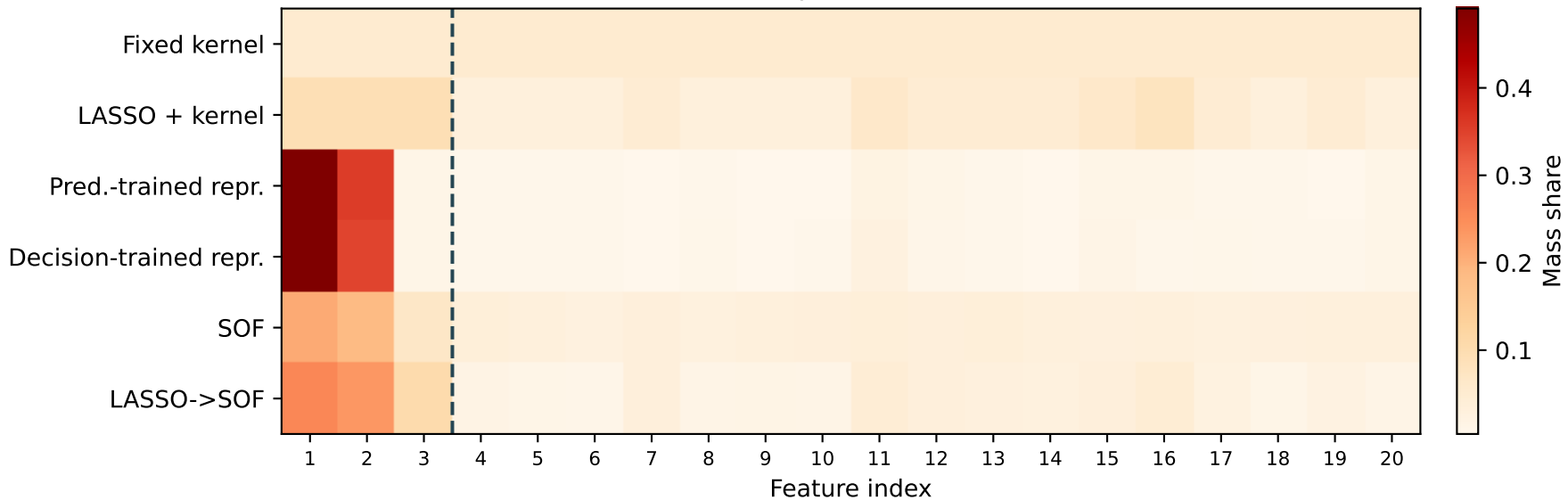
Benchmark A: feature emphasis for (d, k, N) = (20, 3, 400)
