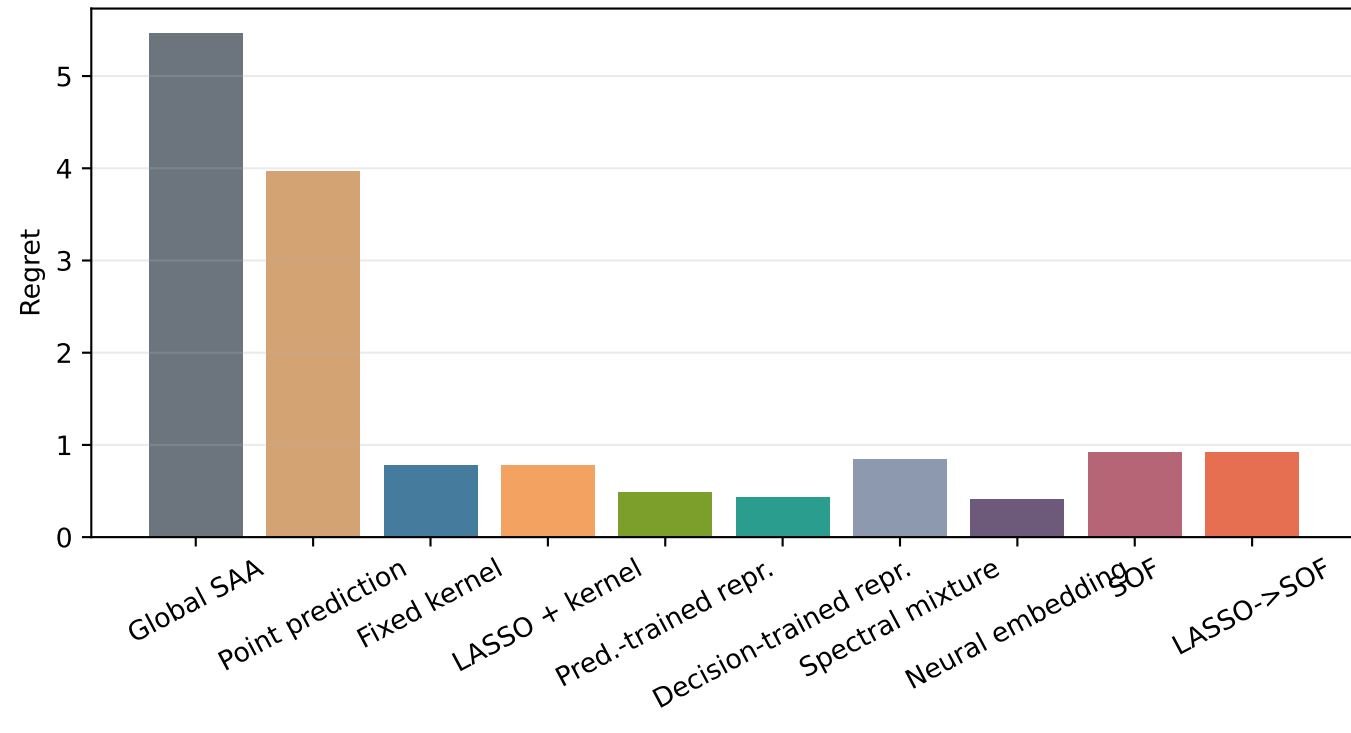
Benchmark B: average regret
