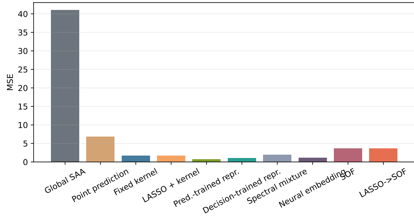
Benchmark B: conditional-mean MSE
