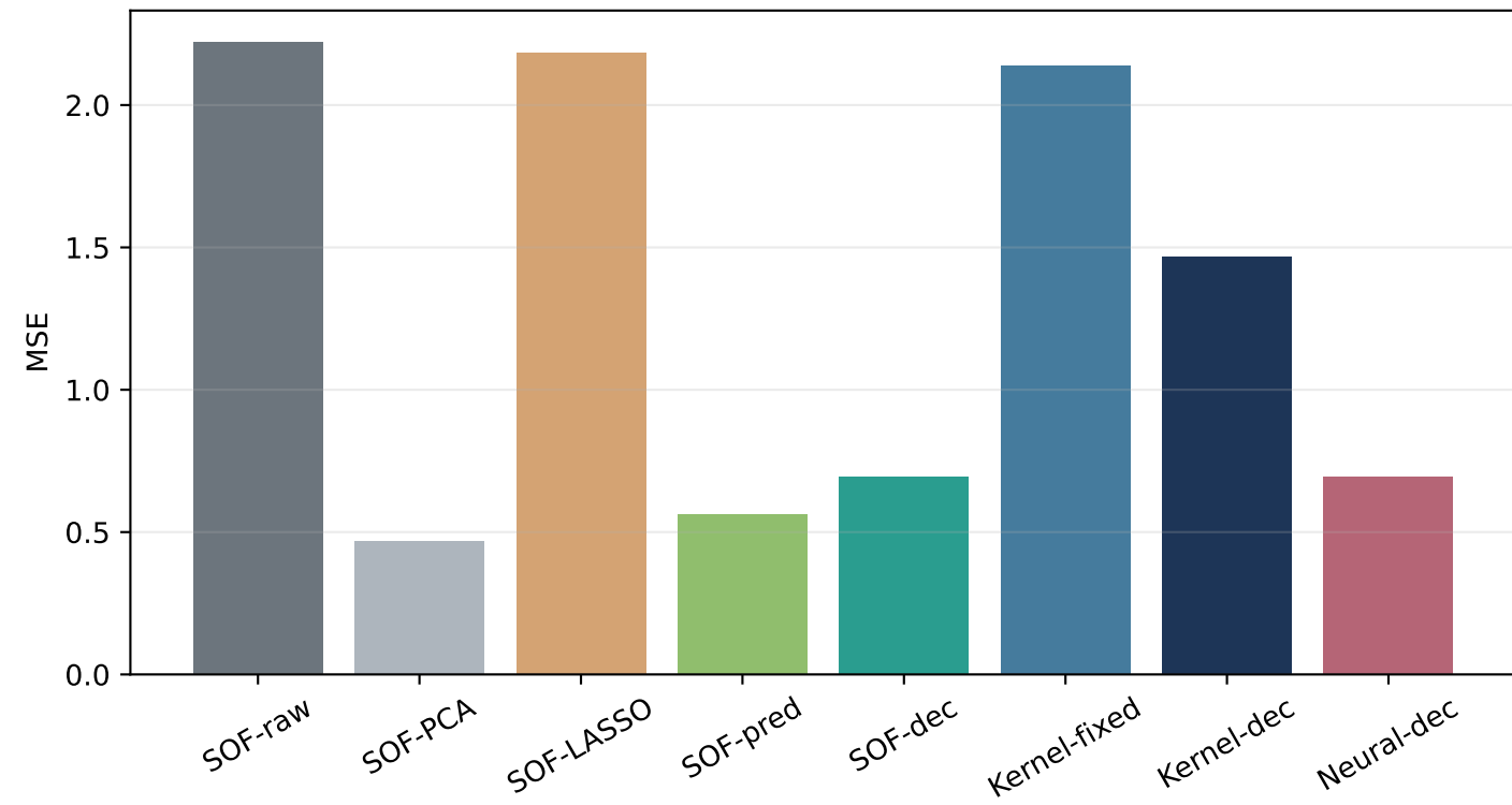
Benchmark C: reward-vector MSE
