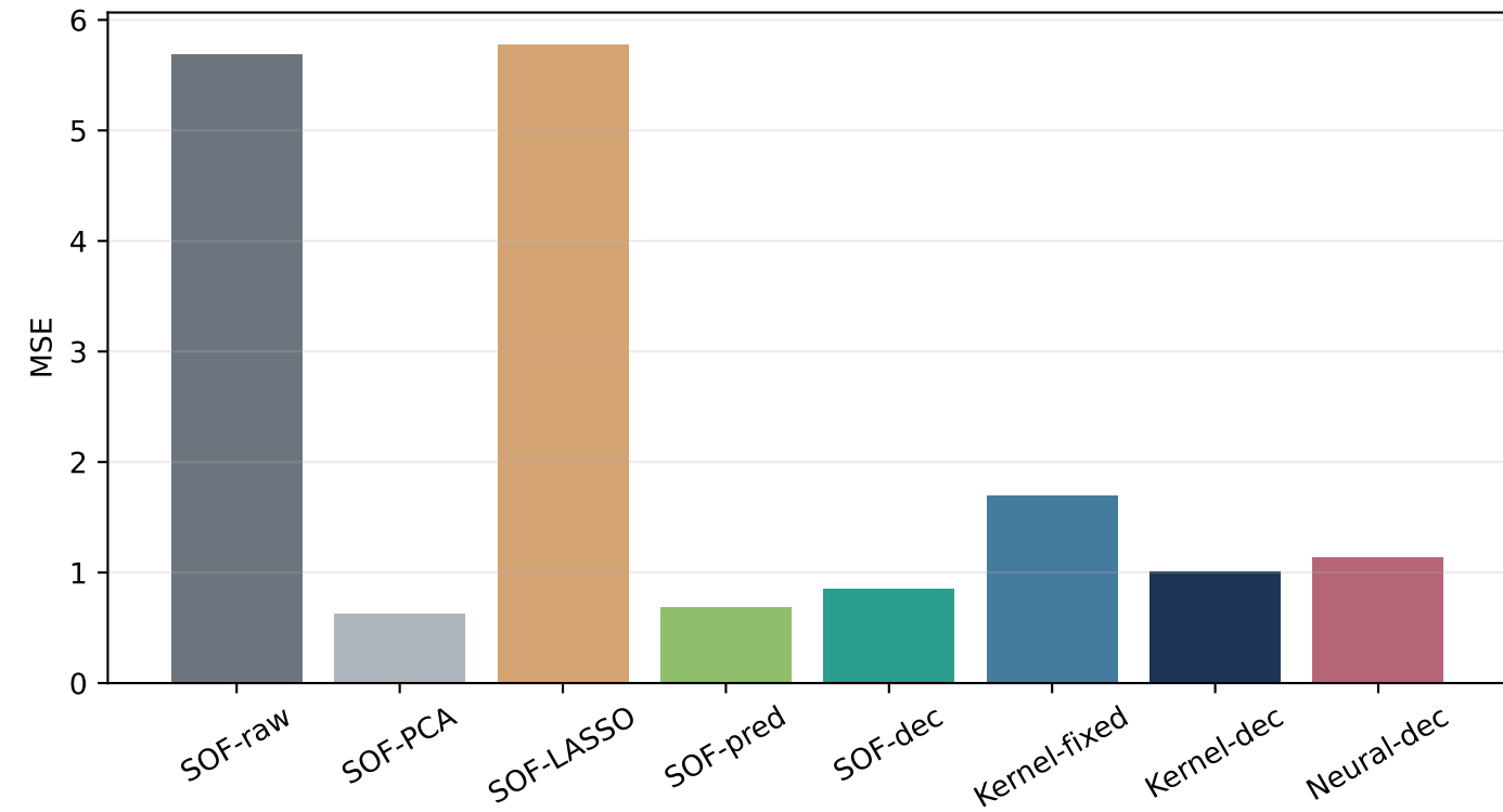
Benchmark C: reward-vector MSE
