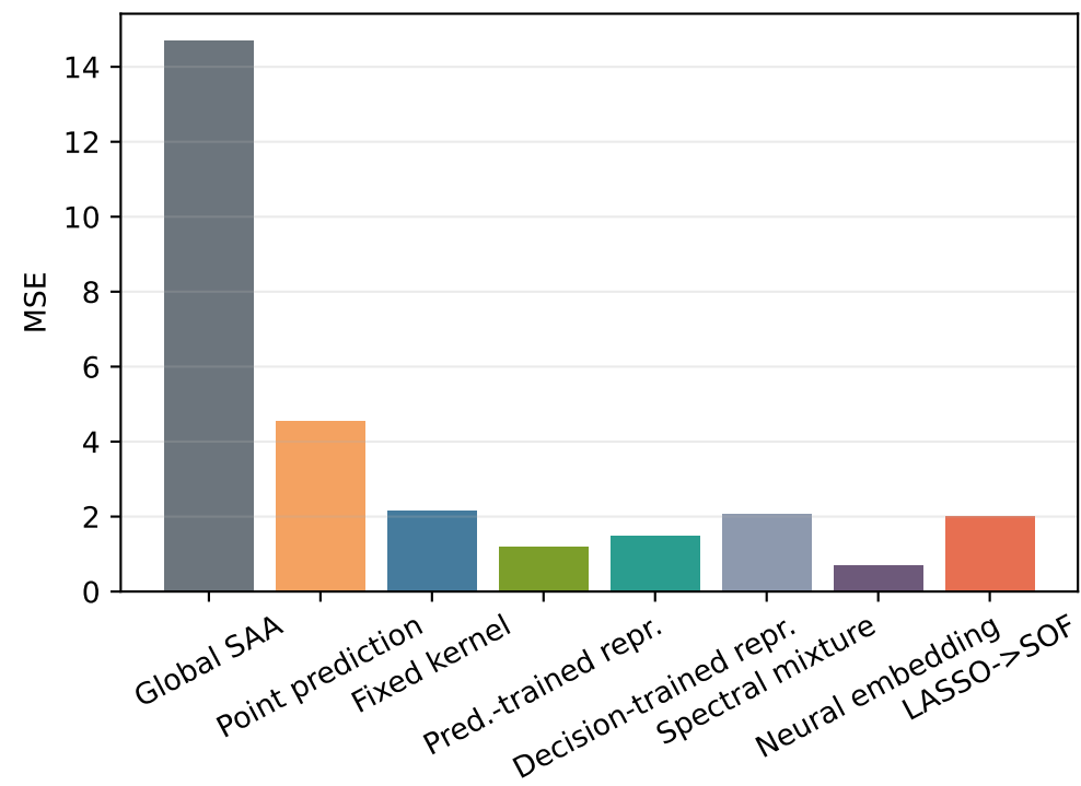
Benchmark C: reward-vector MSE
