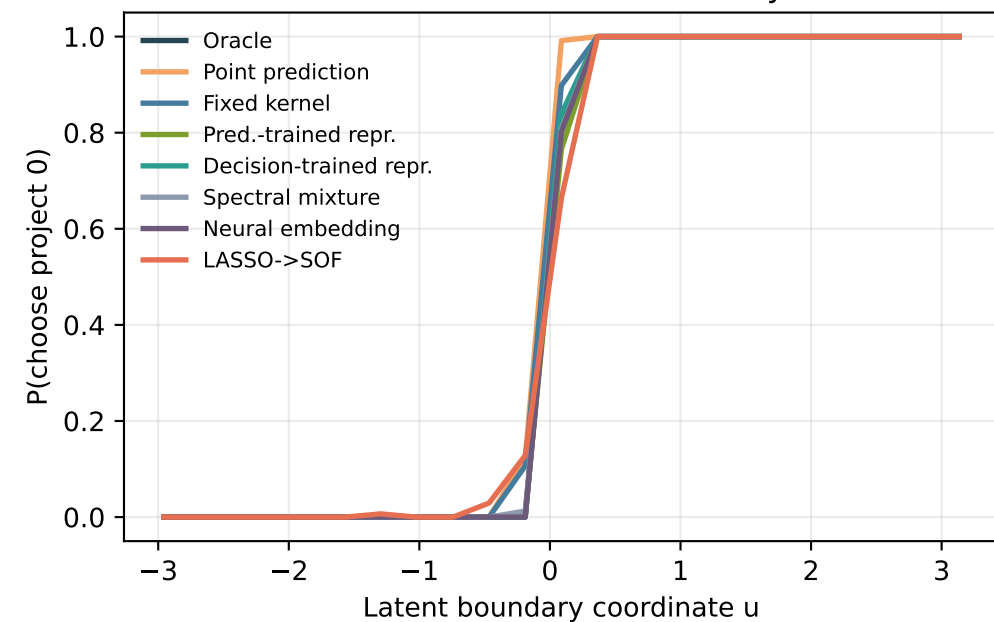
Benchmark C: decision boundary slice
