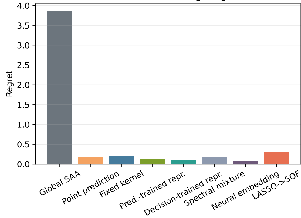
Benchmark C: average regret
