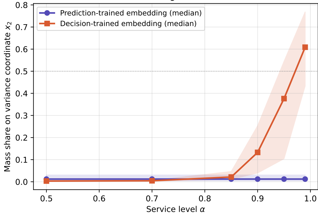
Decision-trained embedding shifts with the cost function
