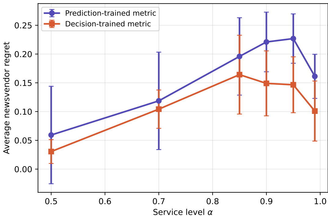
Decision-trained metric tracks the cost function
