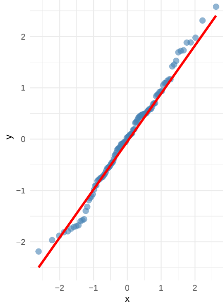
Normal QQ-Plot (RQR)
