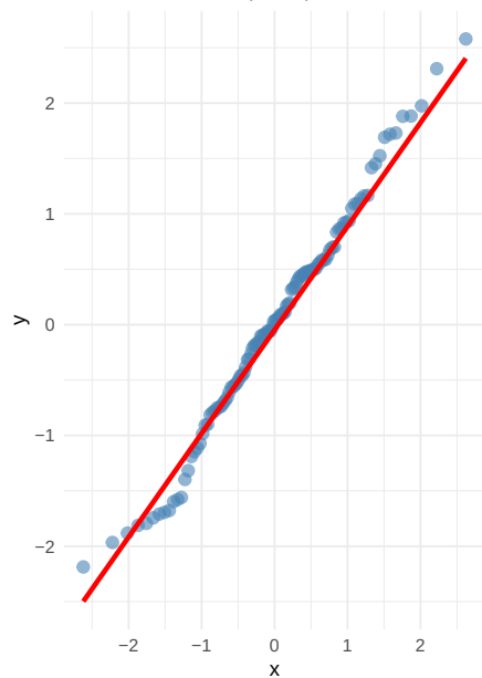
Normal QQ-Plot (RQR)
